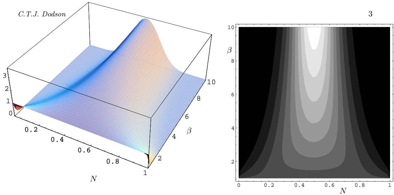
Figure 1: The log-gamma family of densities with central mean \langle N \rangle = \frac{1}{2} as a surface and as a contour plot.
